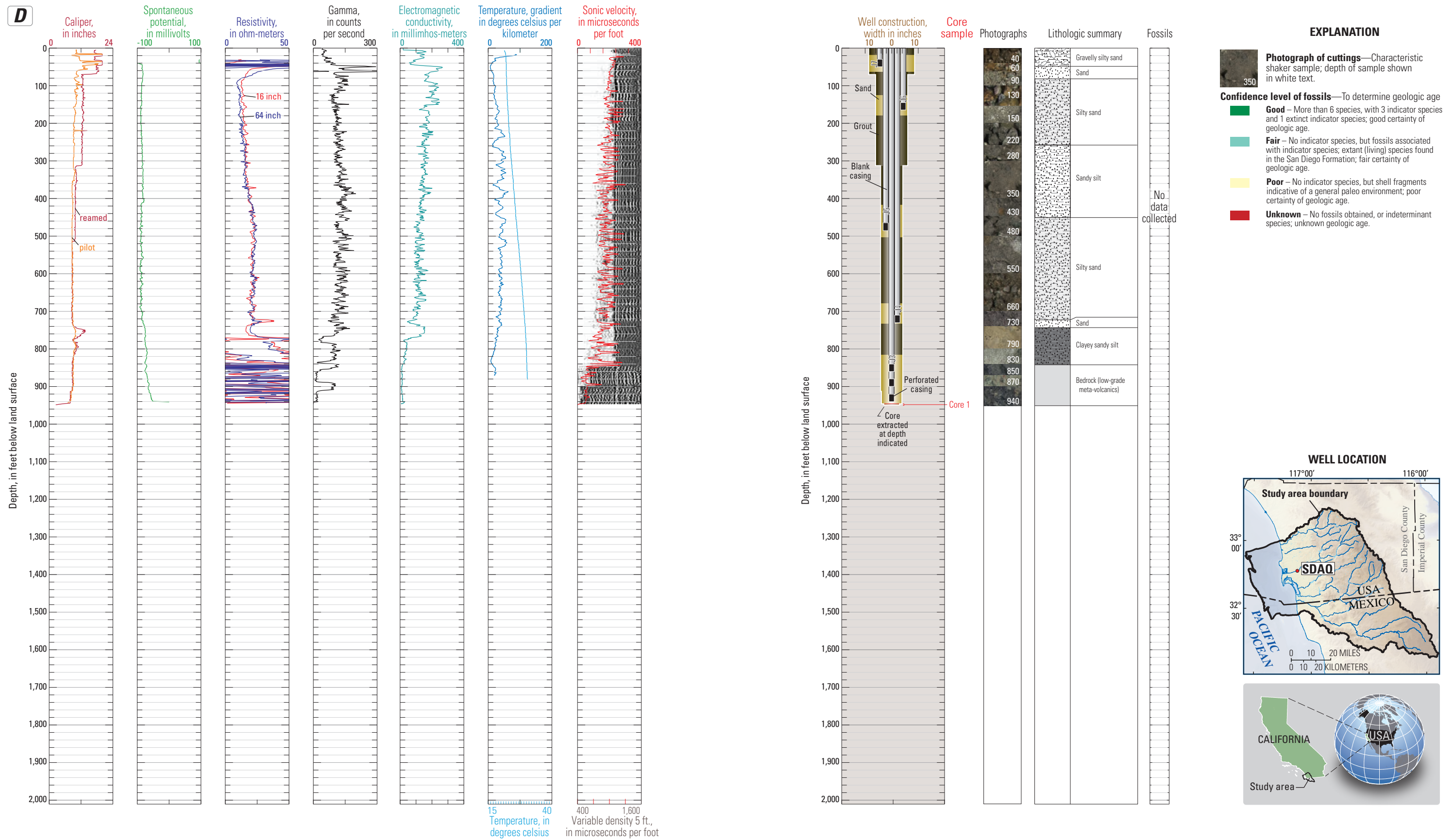
Figure 19D. Well-construction diagrams, generalized lithologic descriptions, and geophysical-log data for caliper, spontaneous potential, resistivity, natural gamma, electromagnetic conductivity, temperature, and sonic logs collected from 16 USGS multiple-depth, monitoring-well sites in San Diego County, California, 1995, 2003–2017: (A) SDCD; (B) SDSY; (C) SDLH; (D) SDAQ ; (E) SDCP; (F) SDBP; (G) SDHF; (H) SDEP; (I) SDNB; (J) SDSW; (K) SDMC; (L) SDLD; (M) SDCC; (N) SDOR; (O) SDOT; and (P) SDBW.—Continued.
